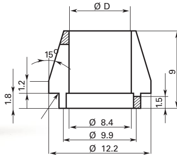
Collets for 8 mm
