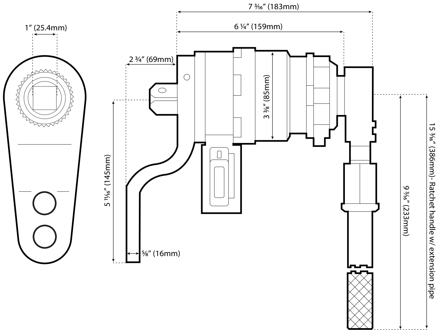
Dimensioned Drawing
