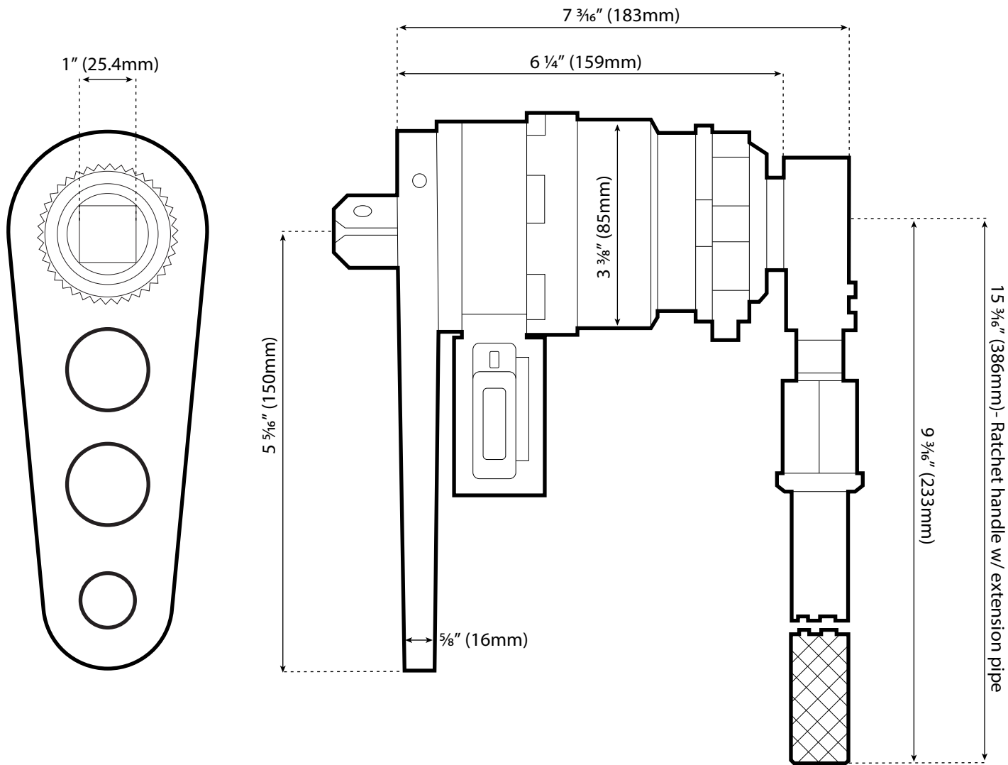
Dimensioned Drawing
