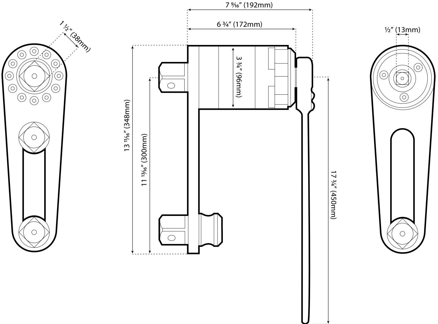
Dimensioned Drawing
