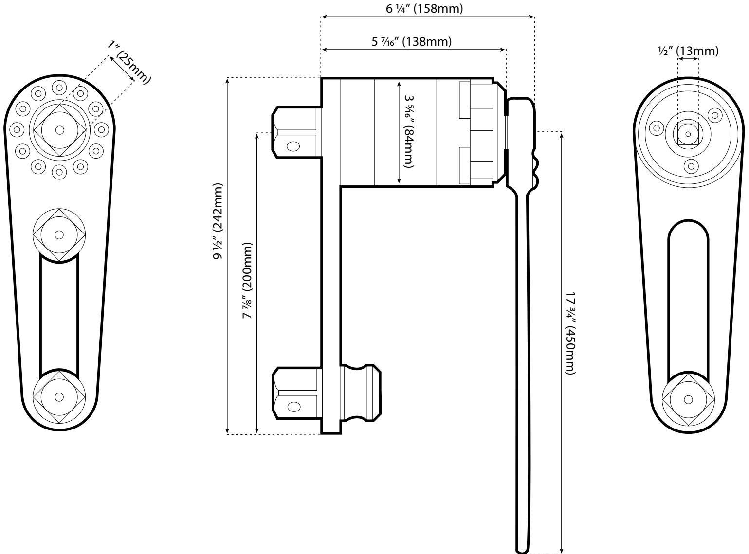
Dimensioned Drawing
