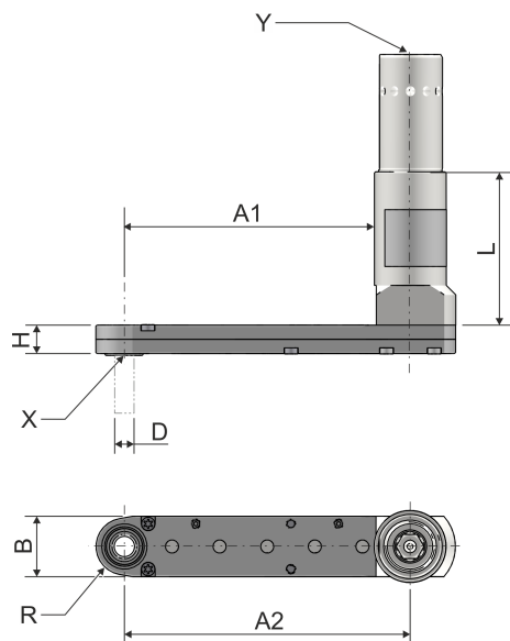
Interface to drilling tool / collet chuck "X"
