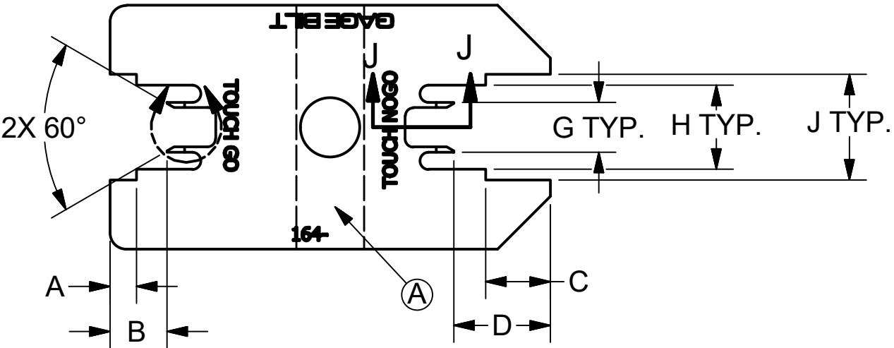
PIN POSITION AND SWAGE GAGE
