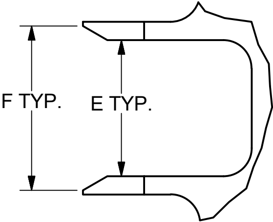
PIN POSITION AND SWAGE GAGE
