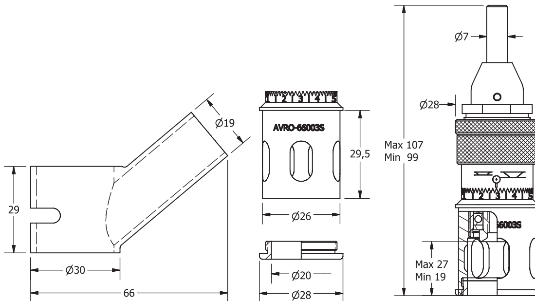
Technical information (mm)
