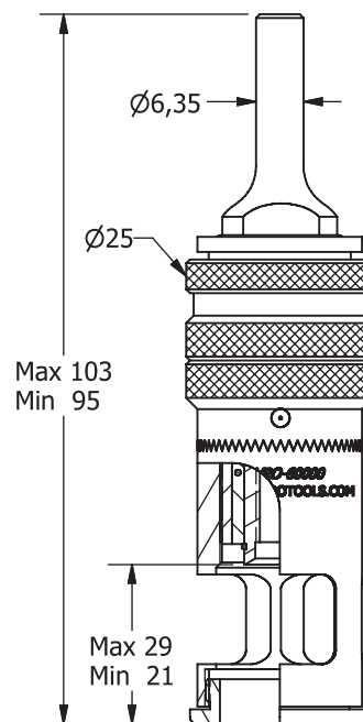
Technical information (mm)
