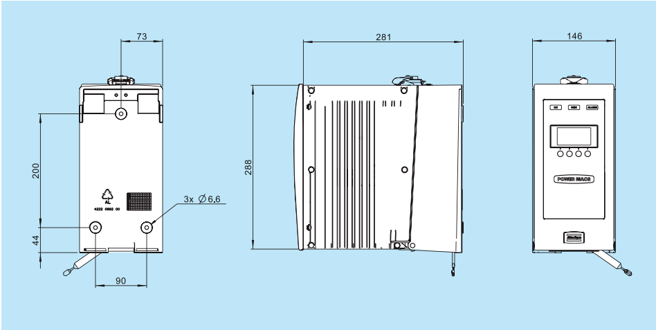
PowerMACS 4000 Secondary TC
