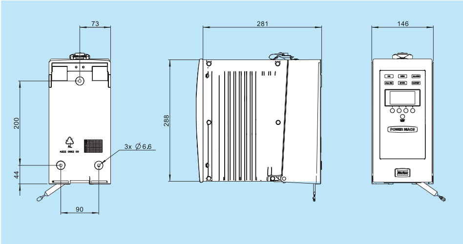
PowerMACS 4000 Secondary TC
