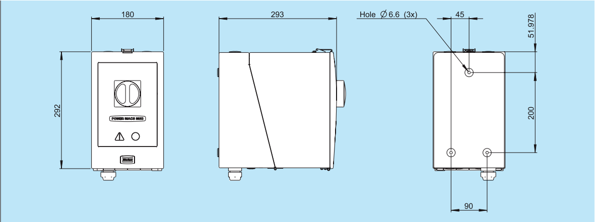
Main switch box
