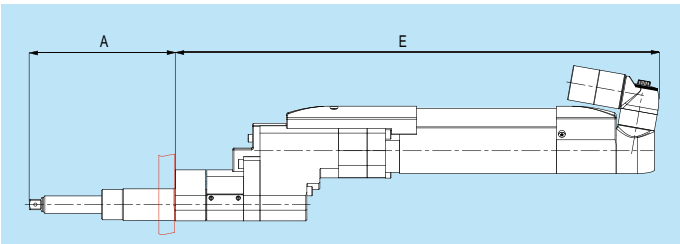
QST – COT & COTT nutrunner
