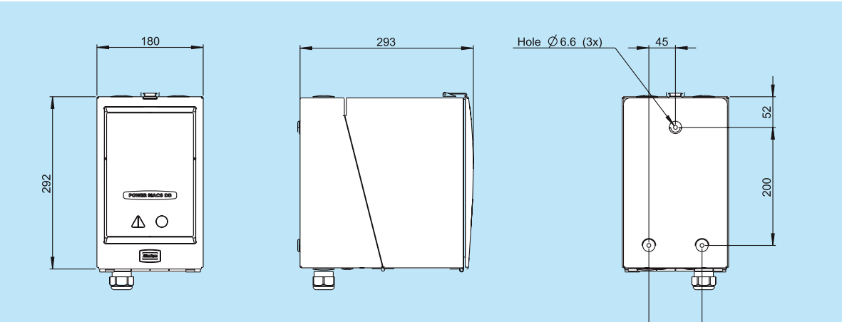
Distribution box
