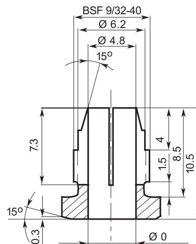
Collets for 5.0 mm (Thread BSF 9/32 -40)
